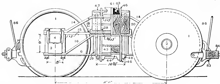
Fig. 4750. Half Side Elevation and Half Longitudinal Section.
